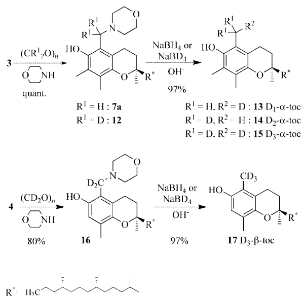
Scheme 3. Preparation of [D 1 ]-, [D 2 ]-, [D 3 ]- \alpha -tocopherols and [D 3 ]- \beta -tocopherol.
