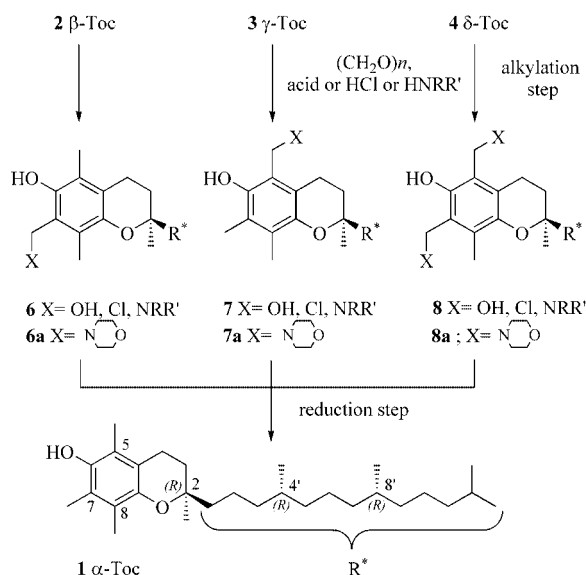
Scheme 1. Two-step alkylation/reduction sequence generally used in the conversion of non- \alpha -tocopherols into 1 . [7]
