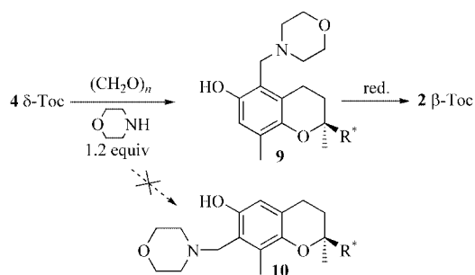
Scheme 2. Regioselective preparation of 2 from 4 .
