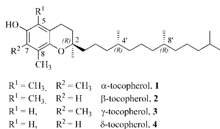
Figure 1. Naturally occurring tocopherols.
